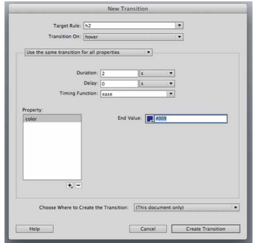
NEW TRANSITION DIALOG BOX
